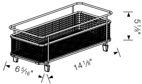
Mesh basket 406399
