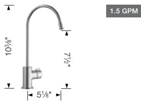
SOLA™ Beverage faucet
