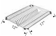
Dish rack 401807
